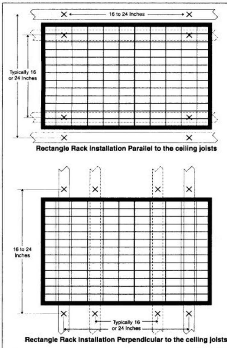
Figure 1 Ceiling Hook Location Guideline
